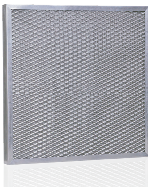
Model: MP-G3-592x592x48 MP: Met Panel G3: Filter Class EN779-2012 592x592x48: Size WxLxD mm
