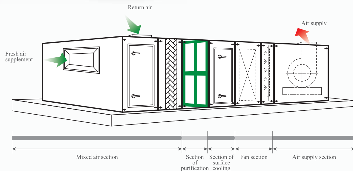
Operating principle of AHU air process
