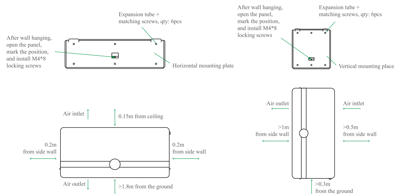
▲ Wall Mounted Type (Horizontal)
